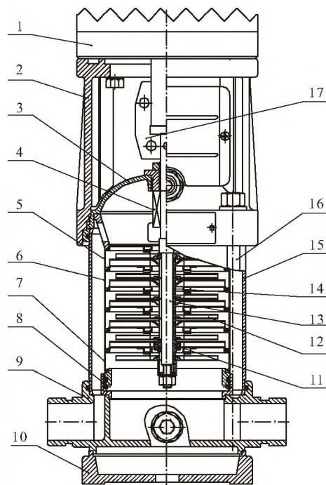
Sectional drawing CDH1,2,3,4
